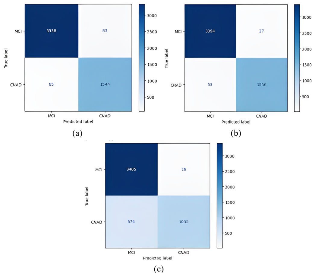
Figure 8 1 vs All classification confusion matrices (MCI/CNAD). (A) EfficientNetB0 model (B) DenseNet121 model (C) AlexNet model.
