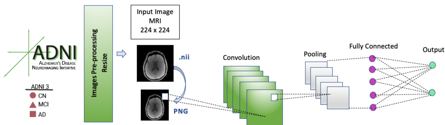
Figure 3 CNN architecture.
