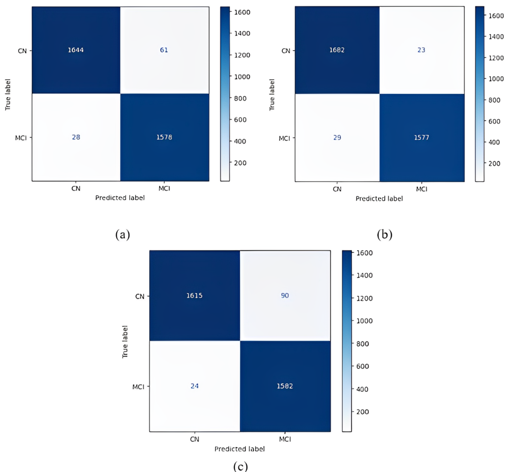
Figure 7 1 vs 1 classification confusion matrices (CN/MCI). (A) EfficientNetB0 model (B) DenseNet121 model (C) AlexNet model.
