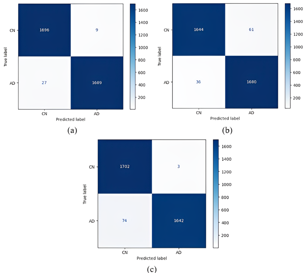
Figure 5 1 vs 1 classification confusion matrices (CN/AD). (A) EfficientNetB0 model (B) DenseNet121 model (C) AlexNet model. Full-size DOI: 10.7717/peerj-cs.1877/fig-5
