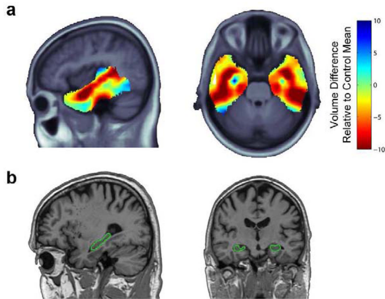
Figure 2. Temporal Lobe and Hippocampal Volume Measures. (a) An unthresholded color-coded map shows the average percent volume reduction of AD patients ( N = 173 ) relative to a standard mean brain image based on identically scanned healthy subjects, in a temporal lobe region of interest overlaid on the population based template. Here the temporal lobe is \sim 10\% smaller in red regions than the average volume in matched controls. The average bilateral temporal lobe volume was used as a quantitative phenotype for the genomic association analysis, prior to fine-scale voxel-based genetic association mapping. (b) Automatic delineation of the hippocampus in a representative healthy elderly subject (the hippocampal boundary is shown in green). The average of the left and right hemisphere hippocampal volumes was used as a quantitative phenotype for the genomic association analysis.
