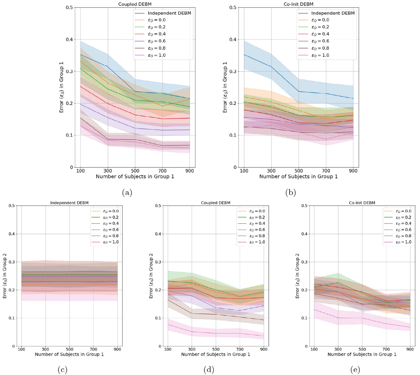
Fig. 4. Experiment 1: The effect of \varepsilon_0 (the difference in groundtruth event orderings in the two groups) on the performance of the proposed methods. The shaded region in these plots represents standard deviation of the error in estimation of the proposed methods in 50 random iterations of simulations. The plots in (a) and (b) show the ordering errors in Group 1 using Coupled DEBM and Co-init DEBM with independent DEBM shown in both (a) and (b), as a function of number of subjects in Group 1. The plots in (c), (d) and (e) show the ordering errors in Group 2 using independent DEBM, Coupled DEBM and Co-init DEBM respectively as a function of number of subjects in Group 1.
